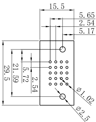
P.C. Body Hole Layout
